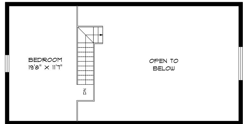
SECOND FLOOR 311 SQUARE FEET
