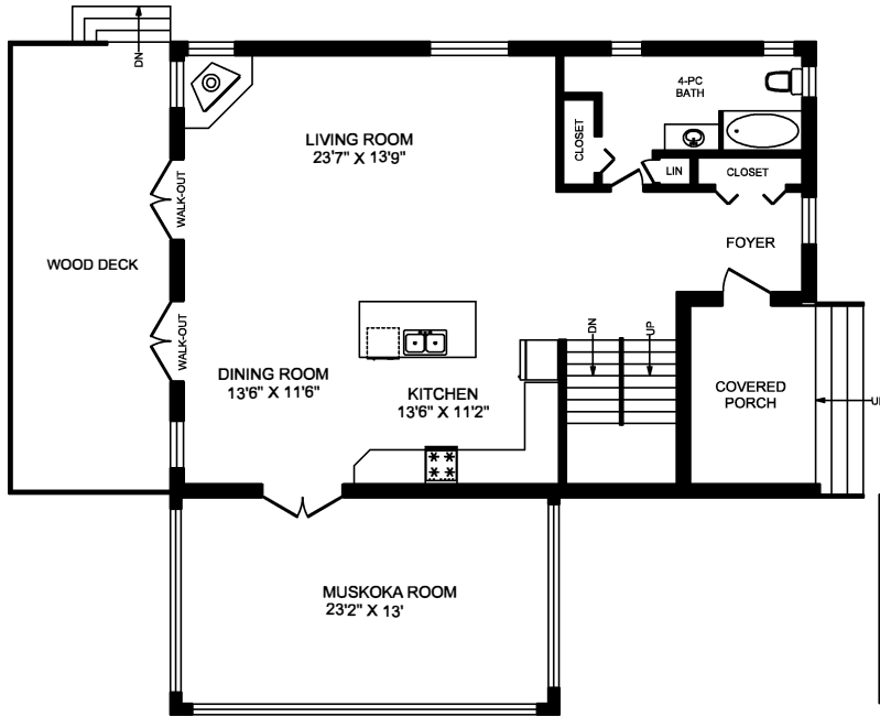
MAIN FLOOR 1412 SQUARE FEET
